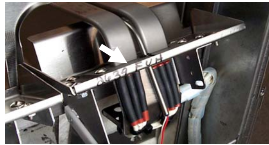
Figure 3: A shroud is provided in the retrofit kit and should be added if the raised edge (shown with the arrow) is absent from the fryer being retrofitted. A tilt-plate without the needed shroud is shown below.
