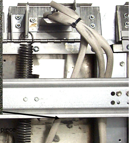
Figure 1: A fryer exhibiting these features will require a complete retrofit.
