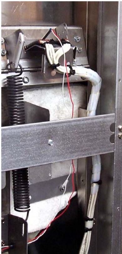
Figure 5: A reworked fryer is shown at left. The element wires are attached to the new element support bracket in four places with wire ties. The element wires are also encased in a spiral wrap from the point they leave the bracket to below the level of the hi-limit. A drawing of the wire routing and placement of the spiral wrap is shown on page 10.
